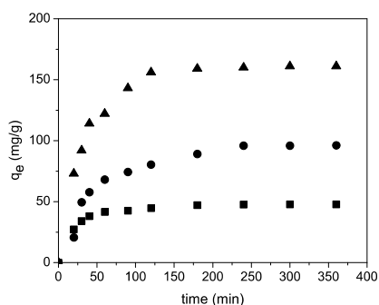
Figure 8. Adsorption kinetics of Red Dye 40 at pH = 3.0, T = 25 °C, and initial dye concentrations of 50 (■), 100 (●), (▲) 200 mg L -1 .
