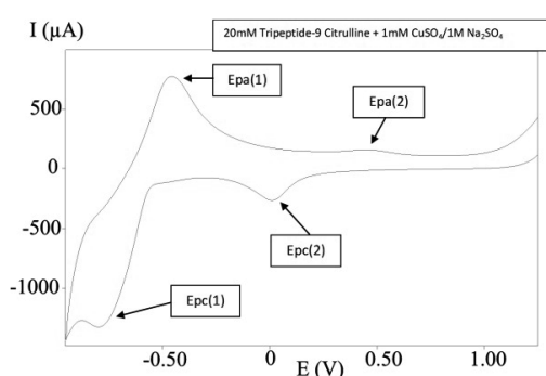
Figure 5. Cyclic voltammograms of Tripeptide-9 Citrulline / CuSO 4 solutions at different concentrations in 1 M Na 2 SO 4 (working solution). 5A , Na 2 SO 4 solution (blank); 5B , 1 mM Tripeptide-9 Citrulline; 5C , 1 mM CuSO 4 ; 5D , 1 mM Tripeptide-9 Citrulline + 1 mM CuSO 4 ; 5E , 2 mM Tripeptide-9 Citrulline + 1 mM CuSO 4 ; 5F , 20 mM Tripeptide-9 Citrulline + 1 mM CuSO 4 . For experimental conditions, refer to "Materials and Methods" section.
