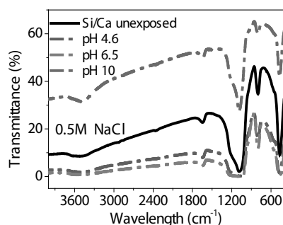
Figure 11. FTIR spectra of Si/Ca pigment after immersion in 0.5M NaCl at different pH values (left) and detail of vibrational band at 616 cm -1 (right).
