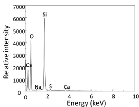
Figure 8. EDAX spectrum and SEM image of Si/Ca pigment after immersion in 0.5M Na 2 SO 4 at pH 10.
