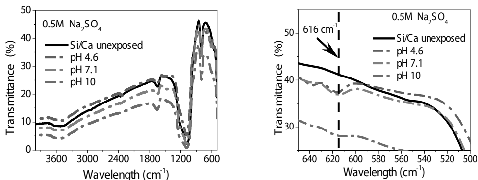
Figure 6. FTIR spectra of Si/Ca pigment after immersion in 0.5M \text{Na}_2\text{SO}_4 at different pH values (left) and detail of vibrational band at 616 \text{ cm}^{-1} (right).
