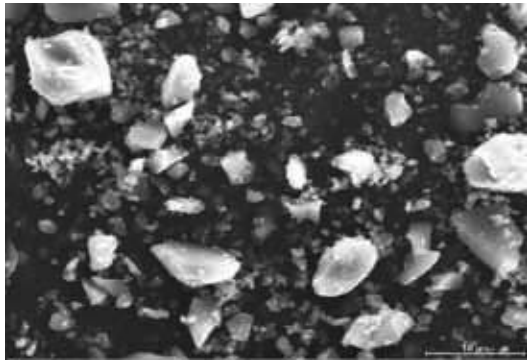
Figure 3. Morphology of Si/Ca pigment particles observed by SEM.
