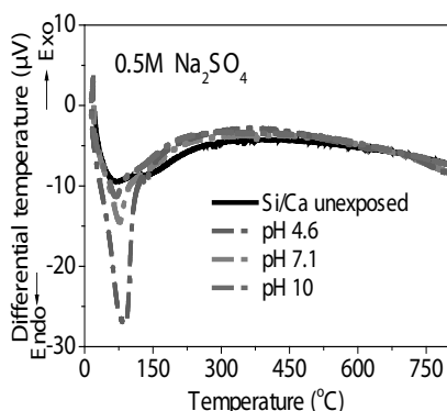
Figure 9. DTA curves for Si/Ca pigment after immersion in 0.5M Na 2 SO 4 (left) and in 0.5M NaCl (right) at different pH values.
