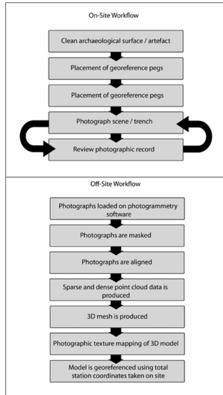
Figure 10. The on-site and off-site workflow for recording archaeological scenes using photogrammetry. On Site: - The surface of the trench is cleaned as usually done prior to photographing. - Placement and georeferencing of pegs with a total station. - The trench (target object) is photographed from as many different angles as possible ensuring at least a 60 percent overlap. - Digital images are downloaded onto a laptop on site and a low resolution model is produced in order to ensure sufficient overlap. Extra photographs are taken if needed. Off Site: - Photographs are loaded into dedicated software where the photos are aligned, and sparse and dense point clouds, 3D mesh and texture of the 3D model are produced. - Once the model is complete, positions of pegs recorded with a total station are tagged to georeference the model within the excavation grid system.
