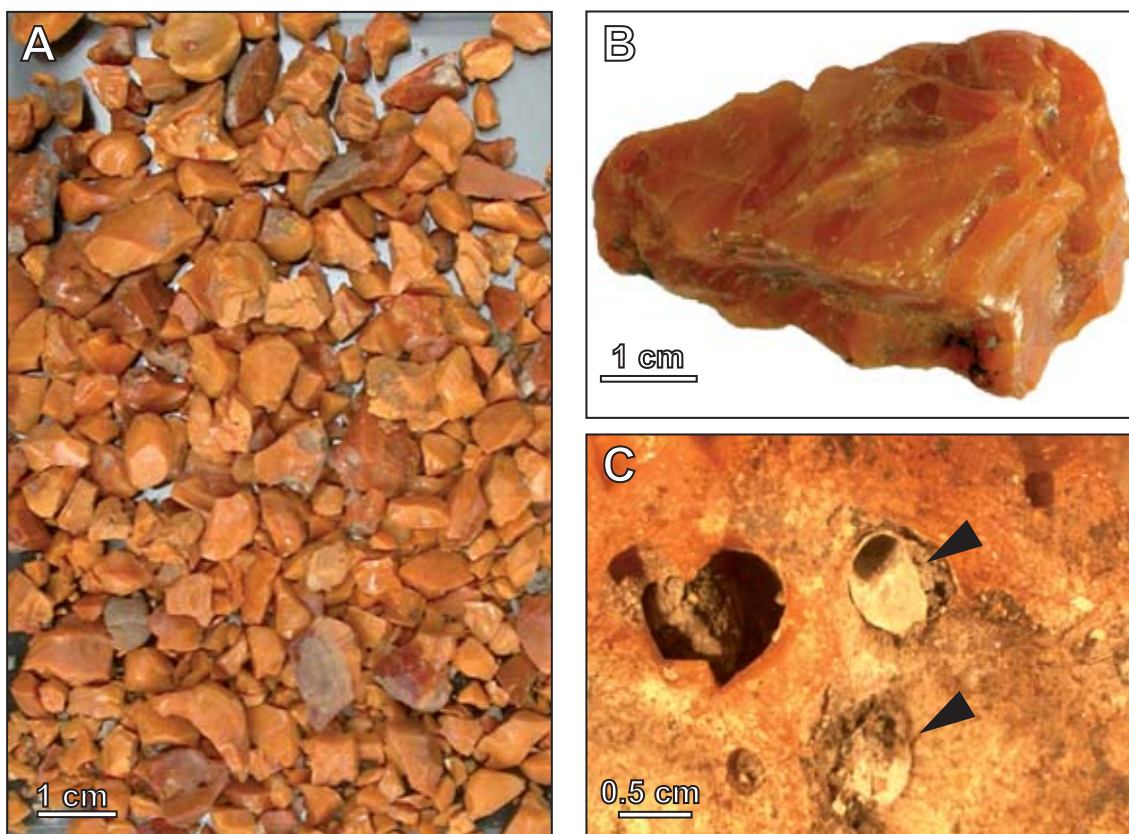
FIGURE 2 | Sarthe amber. A) Amber lumps from Massigné. This material shows the typical characteristics of the Sarthe amber, i.e. its orange colour and its opacity. B) Amber lumps from Écommoy. C) Detail of the surface of an amber lump from Massigné. Note fossil oysters (arrows) attached to the surface, indicating that the Sarthe amber was deposited into a marine or brackish environment.
