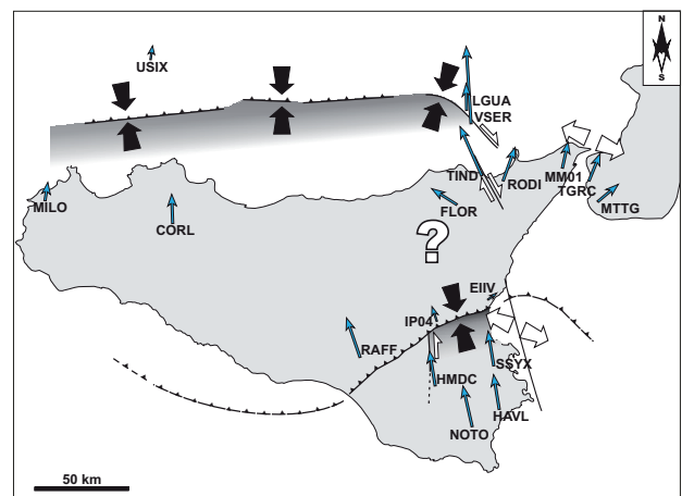
FIGURE 5 | Large scale kinematic model of Sicily. GPS velocity relative to a fixed Eurasian frame are from i) this work (EIIV, IP04, RAFF, HMDC, NOTO, HAVL, SSYX); ii) Mattia et al. (2008 and 2009) (LGUA, VSER, FLOR, RODI, MM01, TIND, TGRC, MTTG) and iii) unpublished data (MILO, USIX, CORL). See Table 1 for details.
