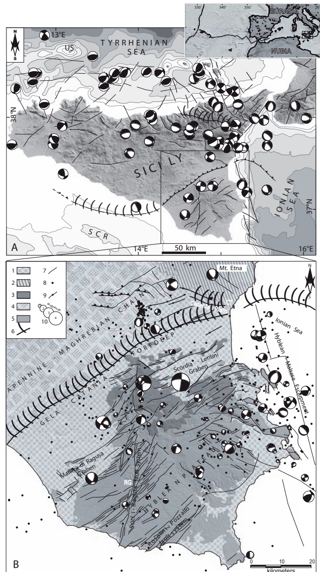
FIGURE 1 | A) Regional tectonic map of the Southern Italy. Focal mechanisms of earthquakes ( M \geq 3.5 ; depth < 40 km) are redrawn from Mattia et al. (2009). Abbreviations are as follow: US: Ustica; SCR: Sicily Channel Rift. The inset shows the Eurasia-Nubia plate tectonic setting. Nubia termed the African plate west of the East African Rift. The plate boundaries are drawn from Bird, (2003). B) Structural sketch map of south-eastern Sicily. 1) Recent-Quaternary sedimentary deposits; 2) Late Pleistocene-Holocene Etnean volcanics; 3) Plio-Pleistocene Hyblean volcanics; 4) Appennine-Maghrebian units; 5) Meso-Cenozoic carbonate sediments; 6) Main thrust fronts; 7) Main faults; 8) Seismic events recorded between 1999 and 2007 ( http://www.ct.ingv.it ); 9) Focal mechanisms selected from Musumeci et al. (2005). Abbreviations are as follow: CT: Catania; RG: Ragusa; Sl: Siracusa.
