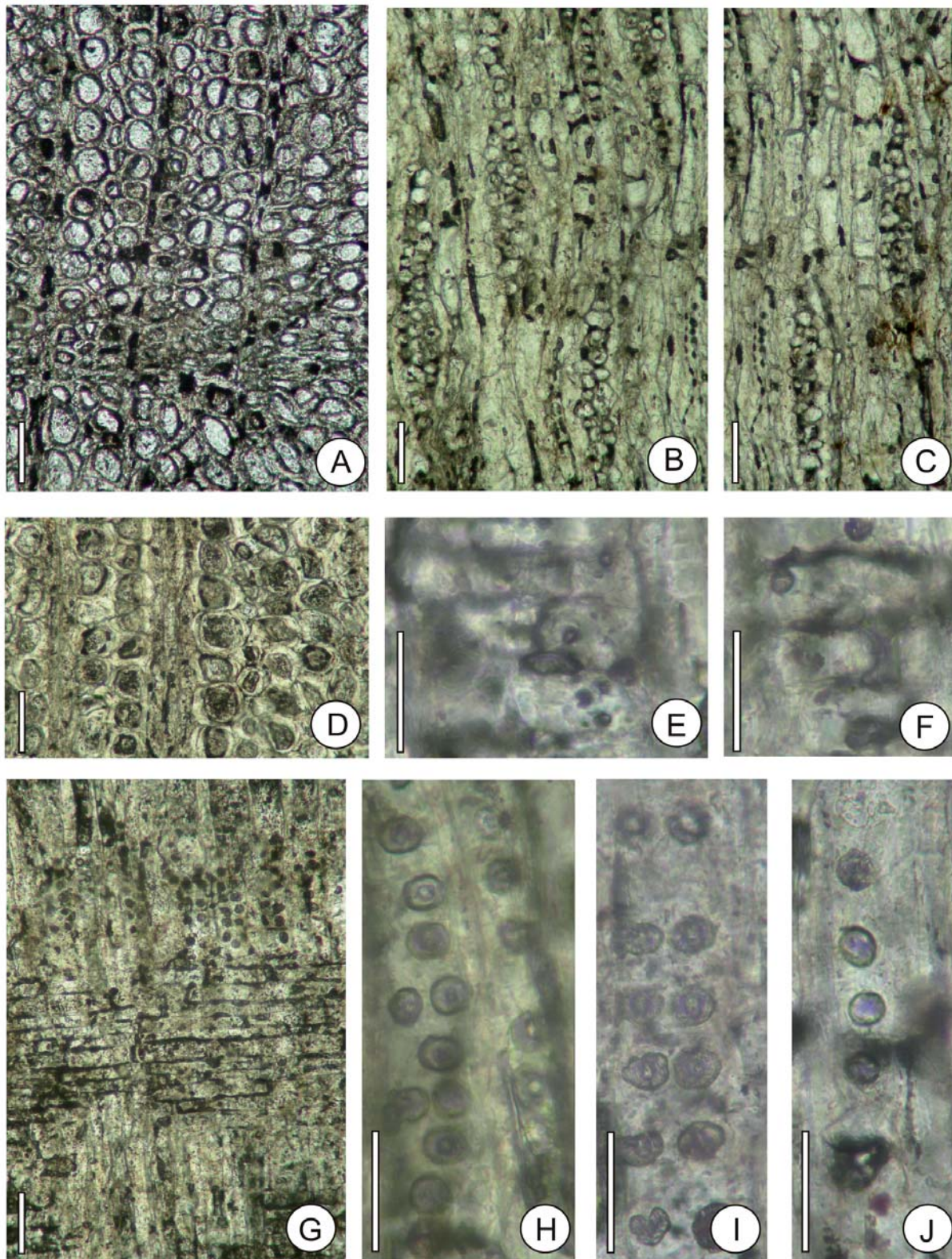
FIGURE 5 | Podocarpoxylon mazzonii . Cross section of the wood to show growth rings. B-C) Tangential section, showing the height, width, and distribution of rays. D) Details of the tracheids and rays in cross section. E-F) Radial section, showing cross fields pits. G) Radial section to show the ray cells, and uniseriate and biseriate bordered pits on the tracheid wall. H-J) Details of uniseriate, partially biseriate and biseriate bordered pits on the radial wall of the tracheids. Note the biseriate the bordered pits are circular or oval, opposite and separate arrangement. Scale bar: 100µm in A-D, G-J; 50µm in E-F. Scale bar: 100µm in A-D, G; 50µm in E-F, H-J.
