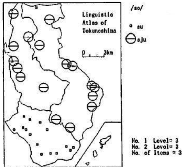
Figure 8. /so/
