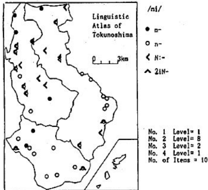
Figure 11. /mi/
