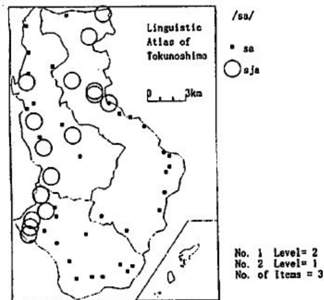
Figure 4. /sa/
