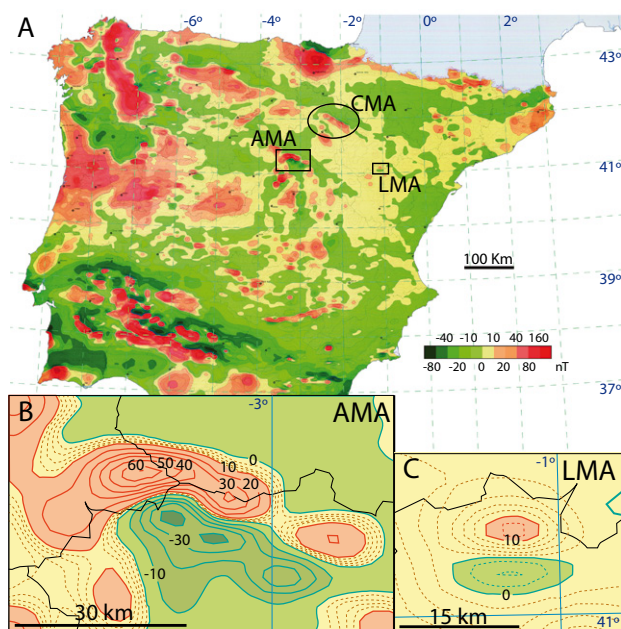
FIGURE 1. A) Magnetic map of the Iberian Peninsula (Socías and Mezcuá, 2002) generated from aeromagnetic data measured in 1987 at an elevation of 3000 m. CMA: Cameros Magnetic Anomaly, AMA: Atienza Magnetic Anomaly, LMA: Loscos Magnetic Anomaly. B) Atienza dipolar anomaly, that can be traced for 45 km along an E-W direction. C) Loscos dipolar anomaly. In C) and B): interval of dashed contours: 2 nT; interval of solid contours: 10 nT.
