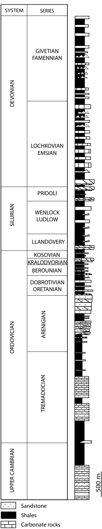
FIGURE 5. Synthetic stratigraphic section of the Palaeozoic materials of the Herrera unit. From Calvin-Ballester and Casas-Sainz, 2014.
