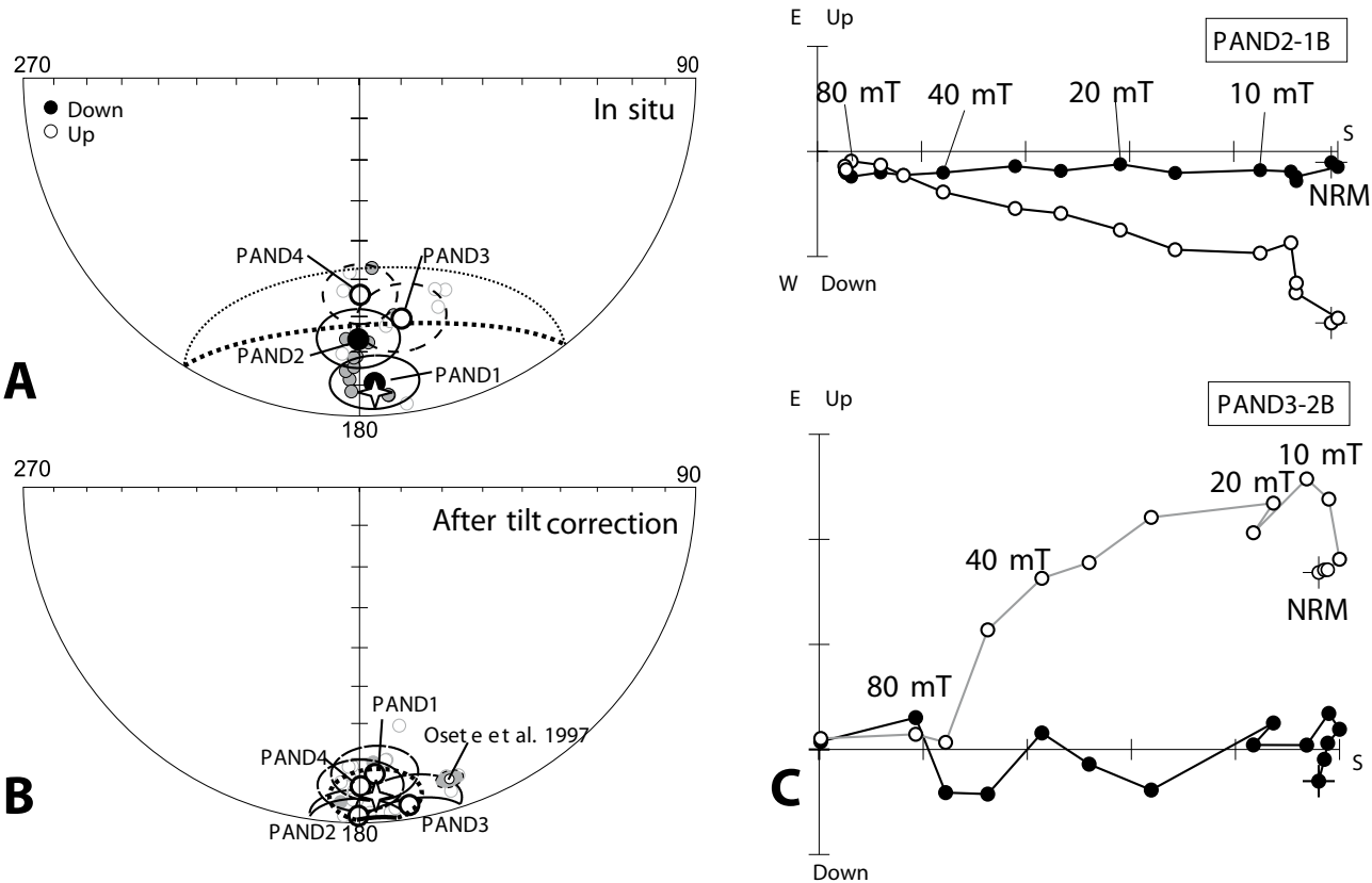
FIGURE 10. A) Equal area projections showing in situ NRM direction of samples (grey) and mean site directions with corresponding 95% confidence circle (black) of four sampling sites in andesites and gabbros. Solid symbols are plotted on lower hemisphere and open symbols on upper hemisphere. Mean of site mean direction is also indicated (star) and the corresponding 95% confidence circles (dotted lines) are also indicated. B) Same information as A), restored to the horizontal assuming that PAND-1 and PAND-2 are located in the northern limb (tilted 25°) of a E-W syncline tilted, while PAND-3 and PAND-4 are located at the southern limb (also tilted 25°). Mean paleomagnetic direction and \alpha_{95} obtained by Osete et al. (1997) in Atienza andesites are also represented. C) Orthogonal projections in in situ coordinates of alternating field demagnetization of two representative samples of andesite (up) and gabbro (down). Open symbols are projections of the vector end points onto the vertical N-S plane and solid symbols are projections onto the horizontal plane.
