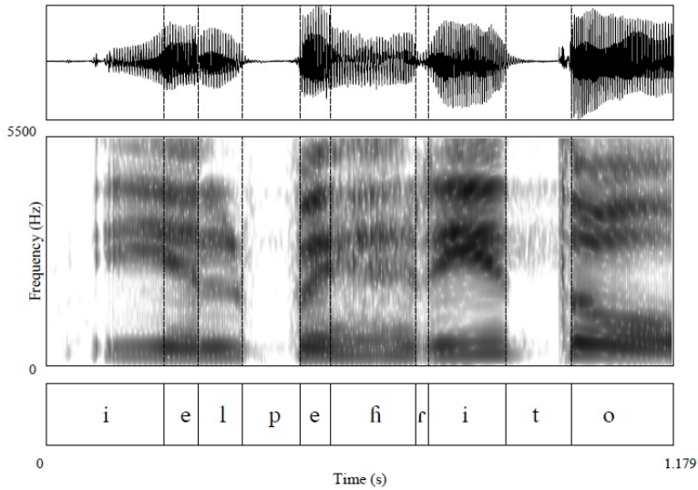
Figure 11. Pre-breathy-voiced tap [ɾ] in DS, with one contact: y el perrito.
