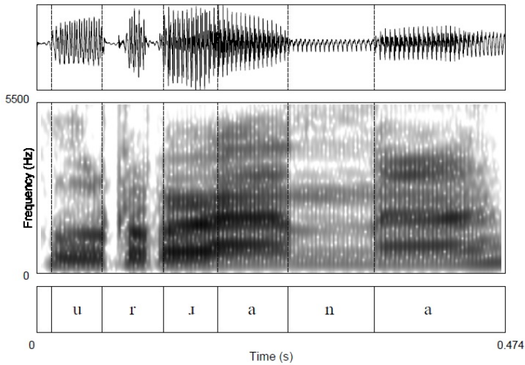
Figure 9. Post-approximantized trill [r] in VMS, with r-coloring: (s)u rana.
