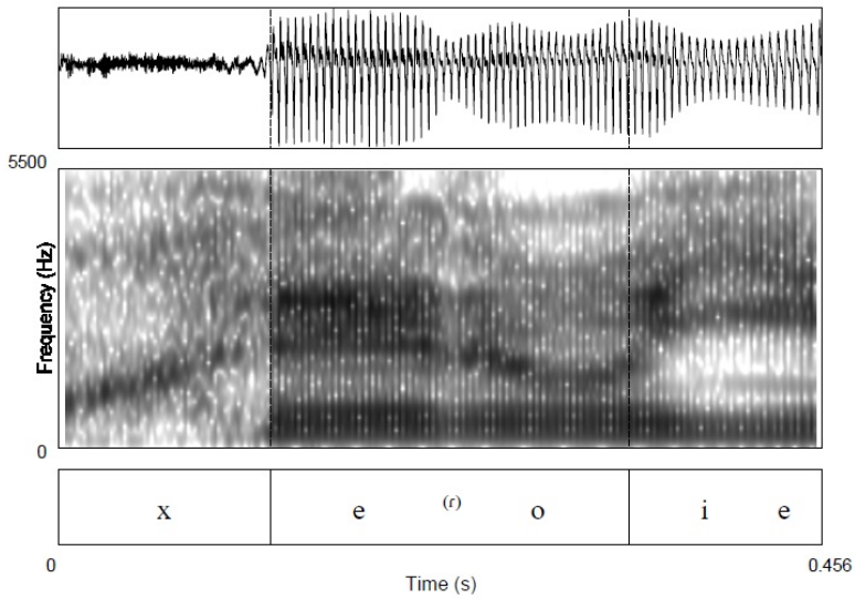
Figure 3. Perceptual tap [ʳ] in VMS: (agu)jero y e(l).
