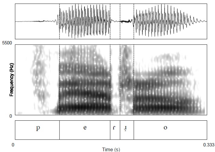
Figure 8. Post-approximant tap [ɾ] in VMS, with aperiodic noise: perro.
