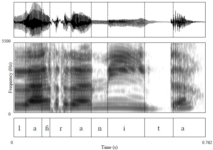
Figure 12. Pre-breathy-voiced trill [r̄] in DS, with three contacts: la ranita.
